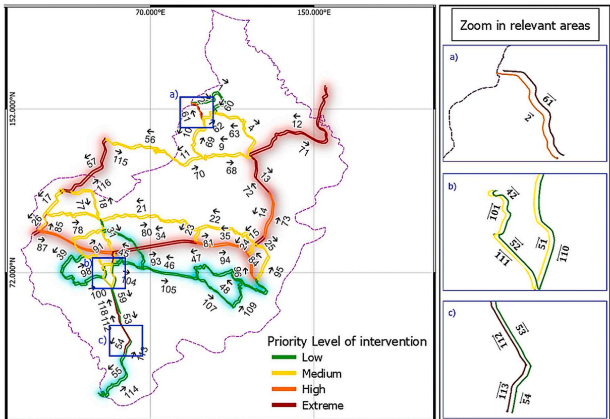
Fig. 13. Priority Level for preparation of the links for the Pedrógão Grande traffic network.
