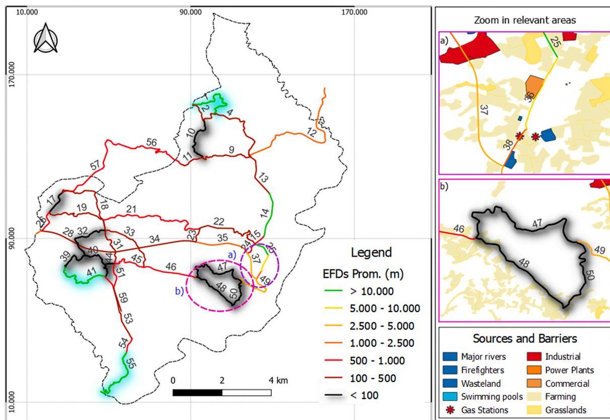
Fig. 8. Equivalent Fire Distances – EFD for Pedrógão Grande Road network (m). Reference burning source: grassland.
